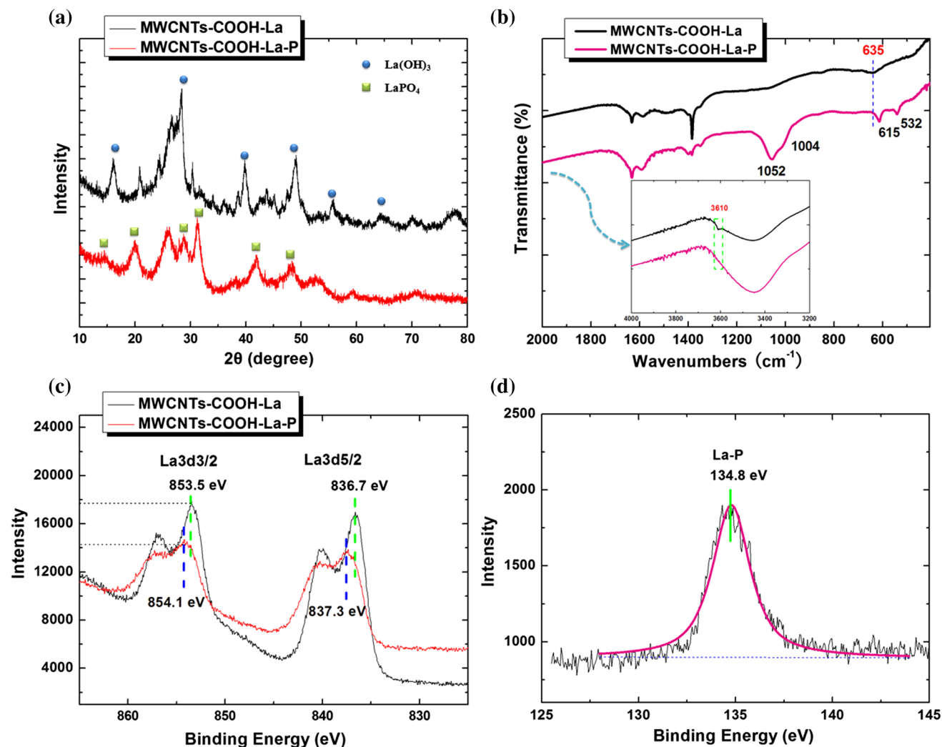
Figure 9 XRD (a), FTIR (b) and XPS spectra of La in the MWCNTs-COOH-La (c) before and after adsorption (MWCNTs-COOH-La-P) and P 2p XPS scan spectrum of MWCNTs-COOH-La-P (d).
