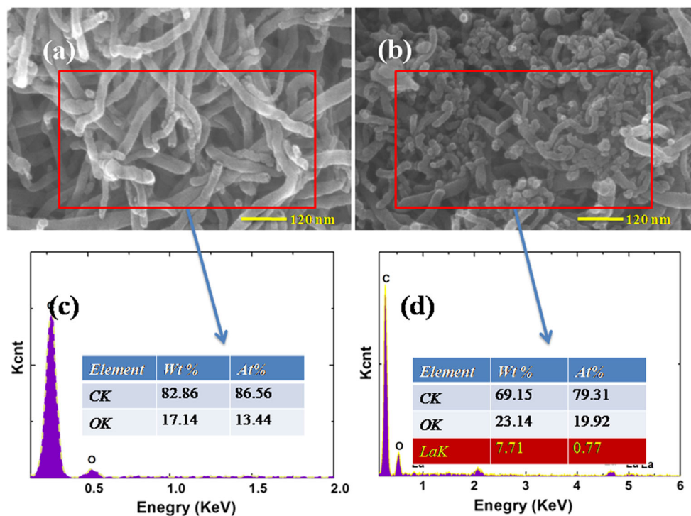
Figure 1 SEM images: a MWCNTs-COOH and b MWCNTs-COOH-La, and EDX of the samples: c MWCNTs-COOH and d MWCNTs-COOH-La.
