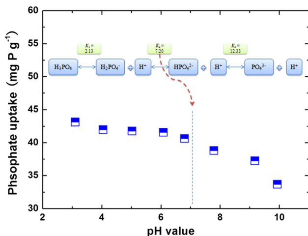
Figure 7 Effect of pH value on phosphate adsorption with the initial phosphate concentration at 50 \text{ mg L}^{-1} , adsorbent dose at 0.625 \text{ g L}^{-1} , at 25 \text{ }^\circ\text{C} .
